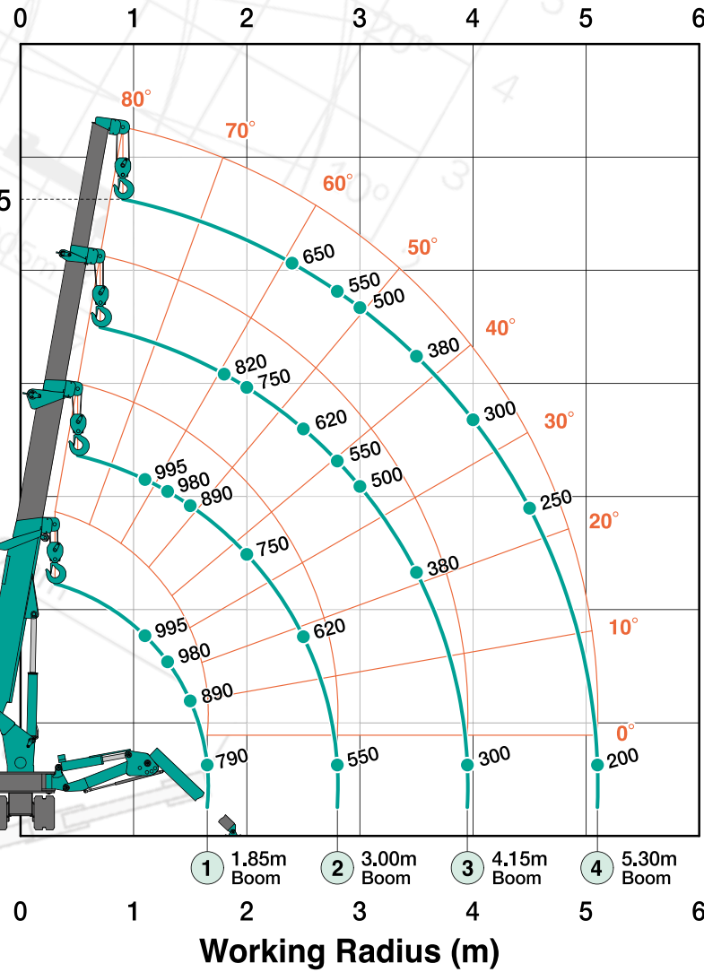
This working range chart shows total rated load including boom deflection.
